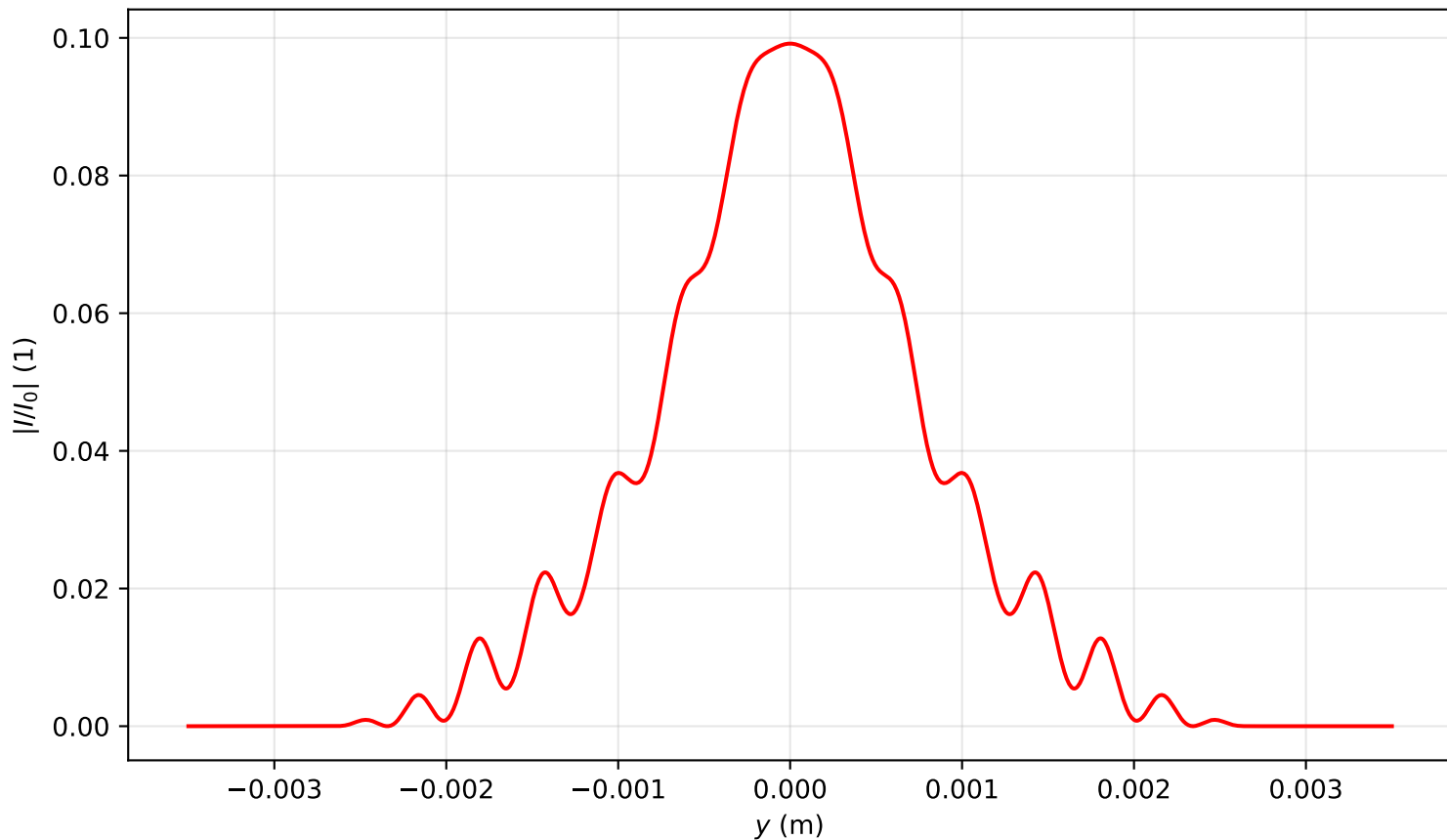
Intensity profile I(x=0, y, z=2.548)/I_0 , P_{in}=2.0P_{cr} , artificial time
